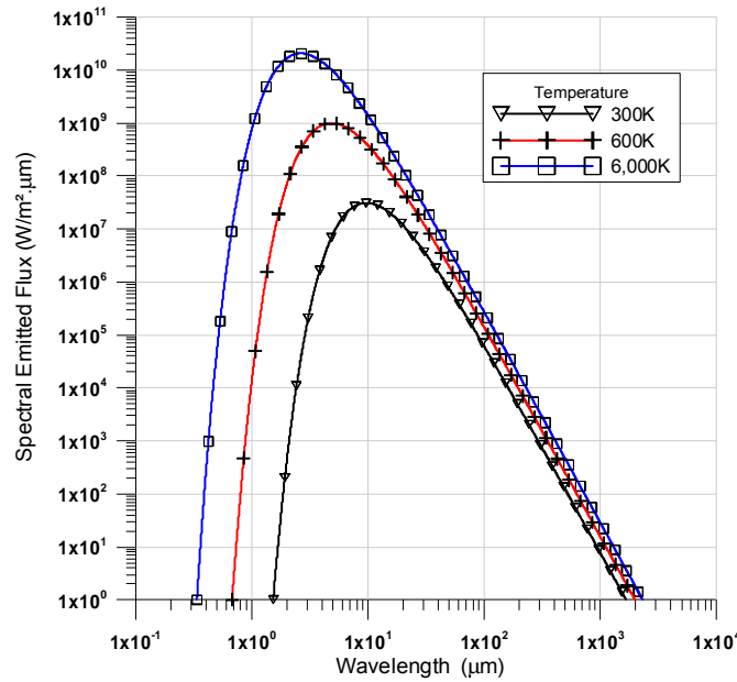
Figure 1- Spectral radiation flux emitted by a blackbody at different temperatures.
